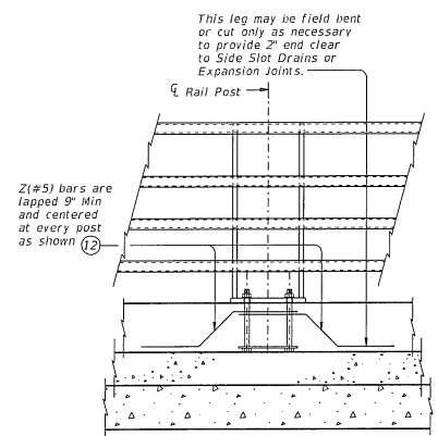
VIEW B-B Bars V and R omitted for clarity. Showing with raised sidewalk.
