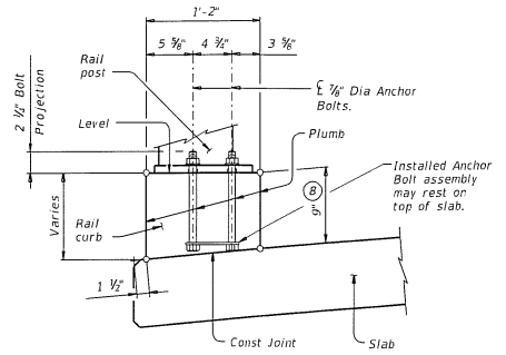
WITHOUT RAISED SIDEWALK
