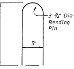
BARS wU(#5)
