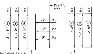
BARS U(#5)
