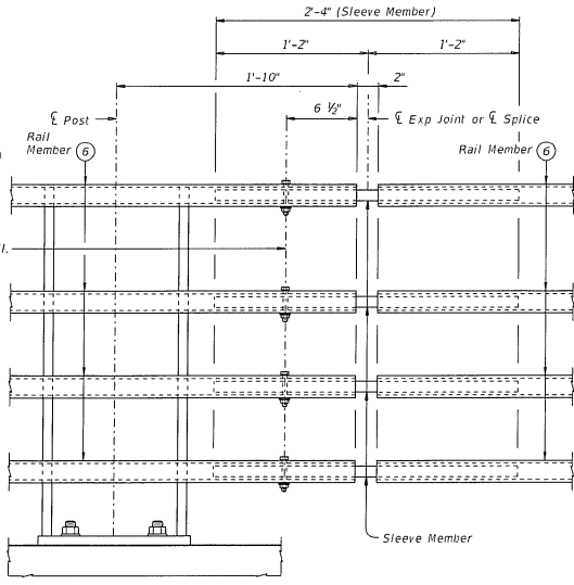
EXPANSION JOINT OR SPLICE
