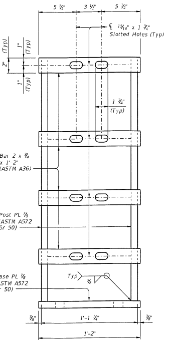
VIEW D-D
