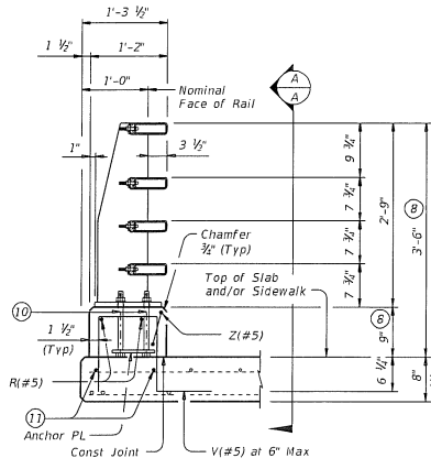
ON BRIDGE SLAB
