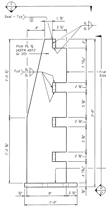
POST DETAIL
