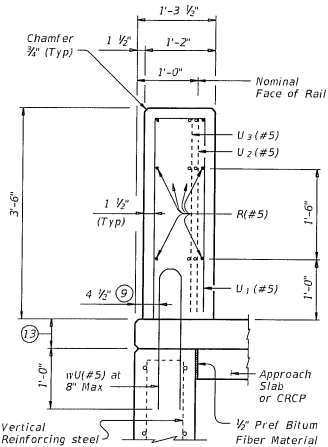
ON ABUTMENT WINGWALLS OR CIP RETAINING WALLS
