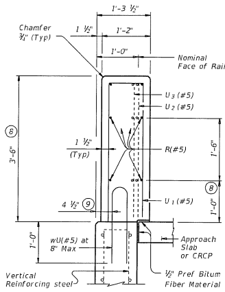
ON ABUTMENT WINGWALLS OR CIP RETAINING WALLS
