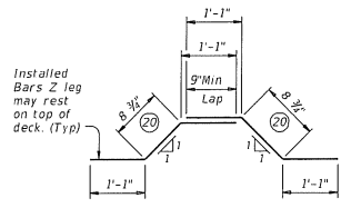
BARS Z(#5)
