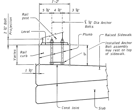
WITH RAISED SIDEWALK
