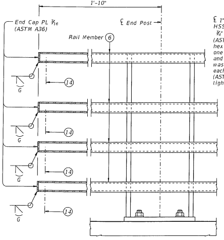
END CAPS ON HSS AT END POST
