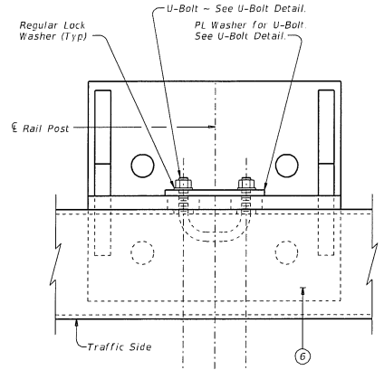
TOP VIEW OF RAIL POST (Showing connection for rail post and HSS.)
